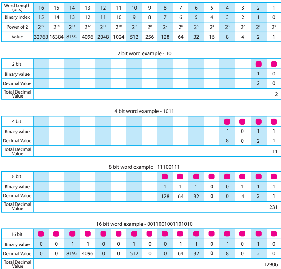
FIGURE 2 - BINARY NUMBER EXAMPLES
