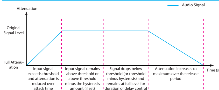
FIGURE 6 - GATE ENVELOPE
