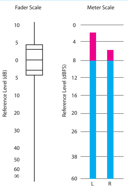
FIGURE 2 - SURFACE DB SCALES
